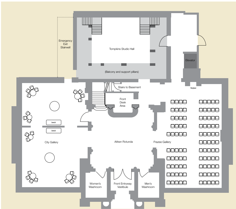
Main level floorplan, with ceremony seating for 101 & cocktail reception setup
